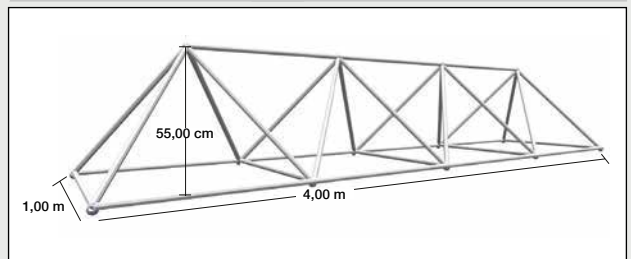
Trellis frame
