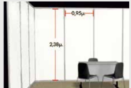
Panel dimensions
